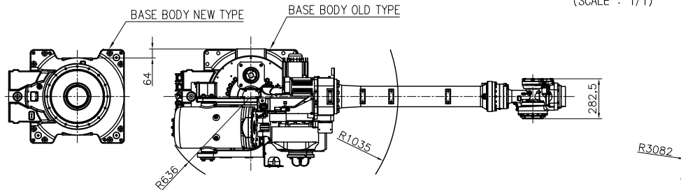
VIEW "B" (SCALE : 1/1)
