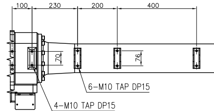
VIEW "E" (SCALE : 2/1)
