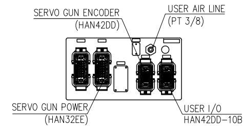
VIEW "C" <For Hi5a Controller> (SCALE : 2/1)
