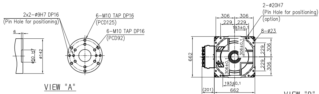
VIEW "B" (SCALE : 1/1)
