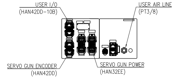
VIEW "C" <For Hi5a Controller> (SCALE : 1/1)
