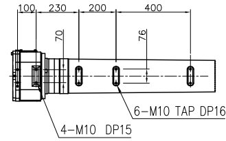
VIEW "E" (SCALE : 1/1)
