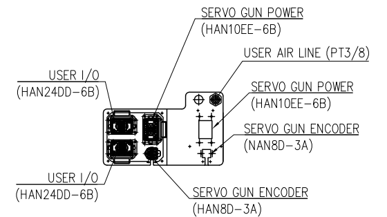
VIEW "D" (SCALE : 1/1)
