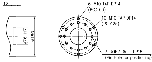
VIEW "A" (SCALE : 4/1)
