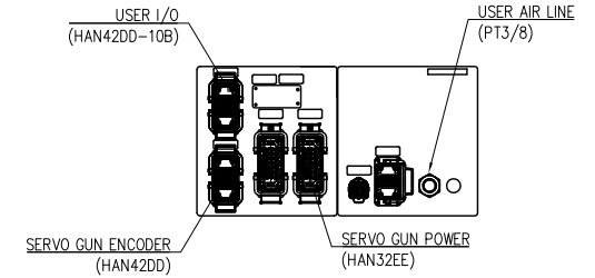
VIEW "C" <For Hi5a Controller> (SCALE : 1/1)
